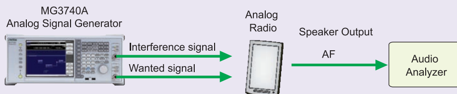
Setup for analog radio Rx characteristics tests
