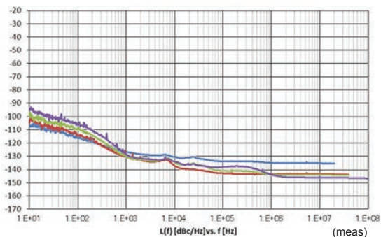
Single sideband phase noise
